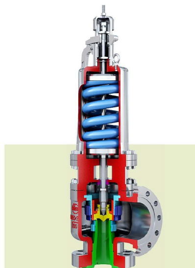
HFA48SB系列高温高压弹簧式安全阀 HFA48SB Series high temperature and high pressure spring safety valve 使用介质: 蒸汽 Medium: Steam Std.:GB/T 12243 Sizes: DN40~250 Press.: PN16 ~ 160 Temp.: -29°C ~ 540°C
