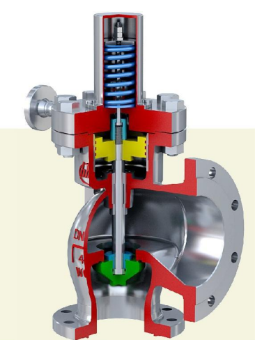
HFA49系列主安全阀 HFA49 Series main safety valve 使用介质: 蒸汽 Medium: Steam Std.:GB/T 12243 Sizes: DN150~250 Press.: PN40 Temp.: ≤425°C
