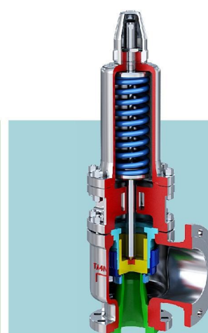
HFA40系列封闭散热器弹簧全启式安全阀 HFA40 Series spring fall lift safety valve with radiator 使用介质: 气体、液体、蒸汽 Medium: Gas, liquid, Steam Std.:GB/T 12243 Sizes: DN40~400 Press.: PN16 ~ 100 Temp.: -196°C ~ 540°C
