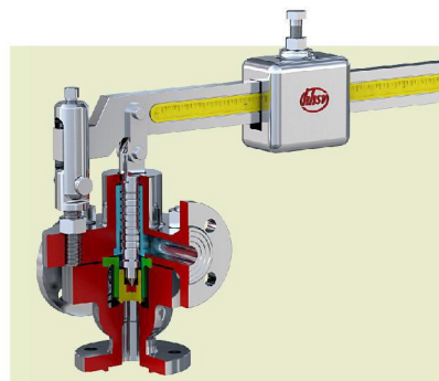
HFGA49 脉冲式安全阀 HFGA49 Series impulse safety device 使用介质: 蒸汽 Medium: Steam Std.:GB/T 12243 Sizes: DN25 Press.: PN40 Temp.: ≤425°C
