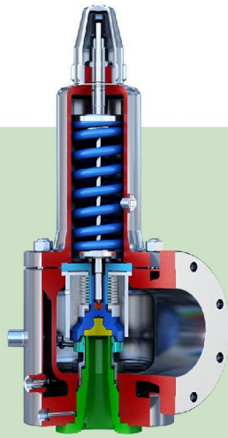
HFNJ系列保温夹套波纹管安全泄压阀 HFNJ Series heating jacket bellows safety relief valve 使用介质: 气体、液体 Medium: Gas, liquid Std.:ASME VIII-API 526 Sizes: 1"-10" Press.: Class 150Lb ~ 600Lb Temp.: -196°C ~ 427°C
