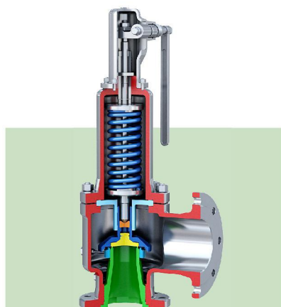
HFA44系列弹簧全启式安全阀 HFA44 Series spring fall lift safety valve 使用介质: 气体、蒸汽 Medium: Gas, Steam Std.:GB/T 12243 Sizes: DN25~400 Press.: PN16 ~ 100 Temp.: -196°C ~ 300°C
