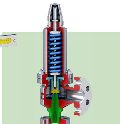
HFA41系列弹簧微启封闭式高压安全阀 HFA41 Series Spring low lift closed high pressure safety valve 使用介质: 气体、液体 Medium: Gas, liquid Std.:GB/T 12243 Sizes: DN15~80 Press.: PN160 ~ 420 Temp.: -196°C ~ 300°C
